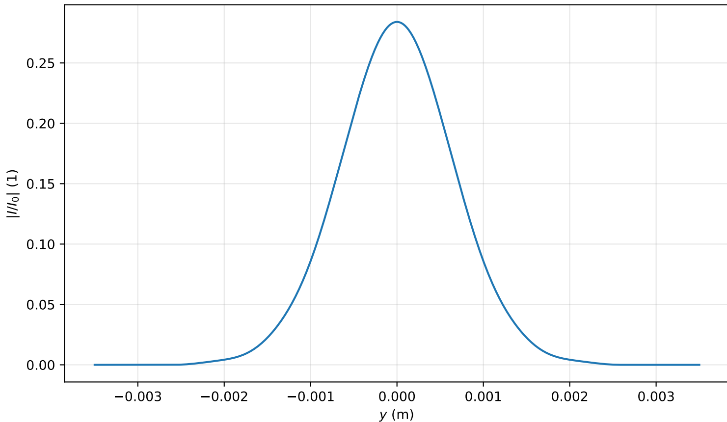
Intensity profile I(x=0, y, z=3.981)/I_0 , P_{in}=0.3P_{cr} , artificial time
